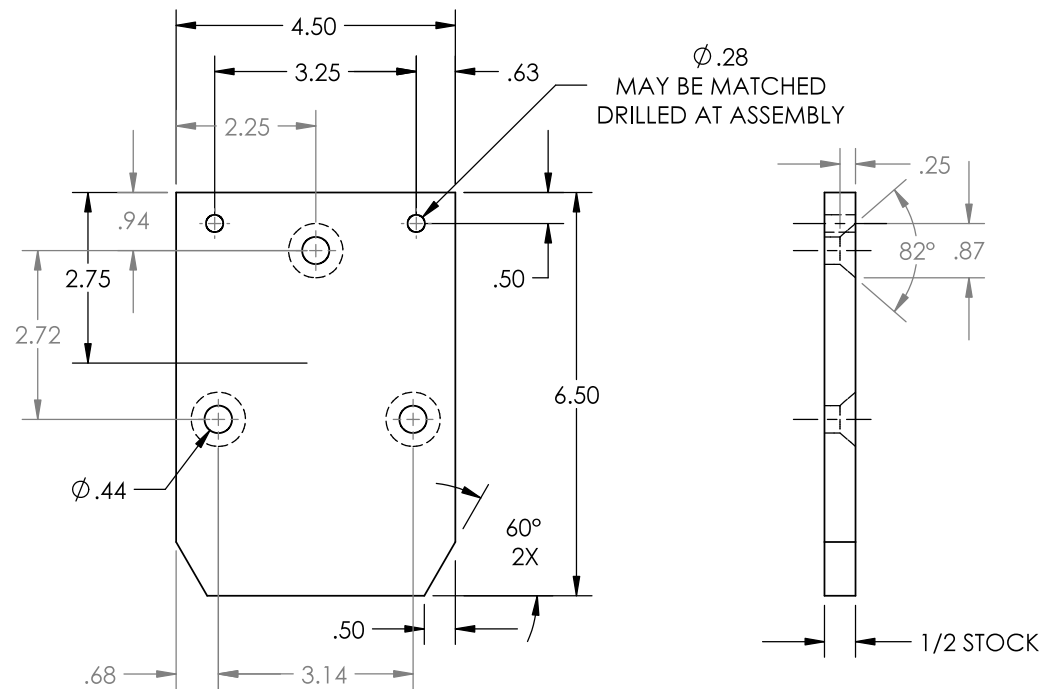
1 110706-99 LOOPBACK PARKING POS CARRIER MATERIAL: 8667K218 1/2 GD G10 FIBERGLASS McMASTER NO. REQ'D: 1
