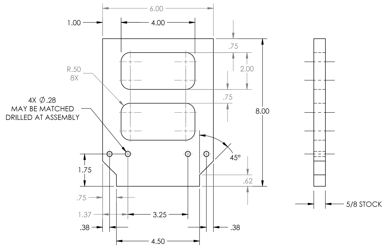
2 110706-98 LOOPBACK PARKING POS CARRIER MATERIAL: 8667K219 5/8 GD G10 FIBERGLASS McMASTER NO. REQ'D: 1
