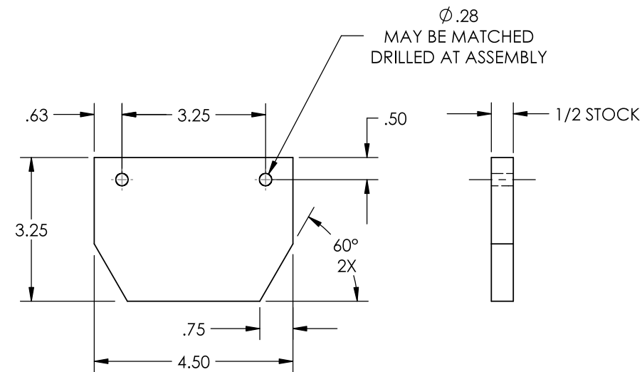
3 110706-97 LOOPBACK PARKING POS CARRIER MATERIAL: 8667K218 1/2 GD G10 FIBERGLASS McMASTER NO. REQ'D: 1
