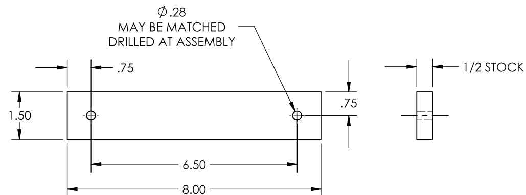
4 110706-99 LOOPBACK PARKING POS CARRIER MATERIAL: 8667K218 1/2 GD G10 FIBERGLASS McMASTER NO. REQ'D: 1
