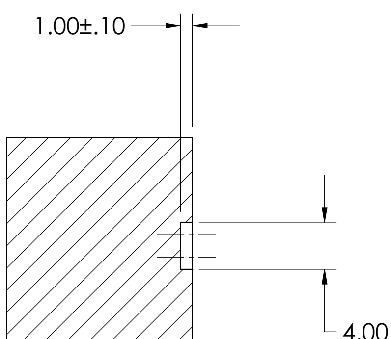
SECTION E-E SCALE 1 : 8
