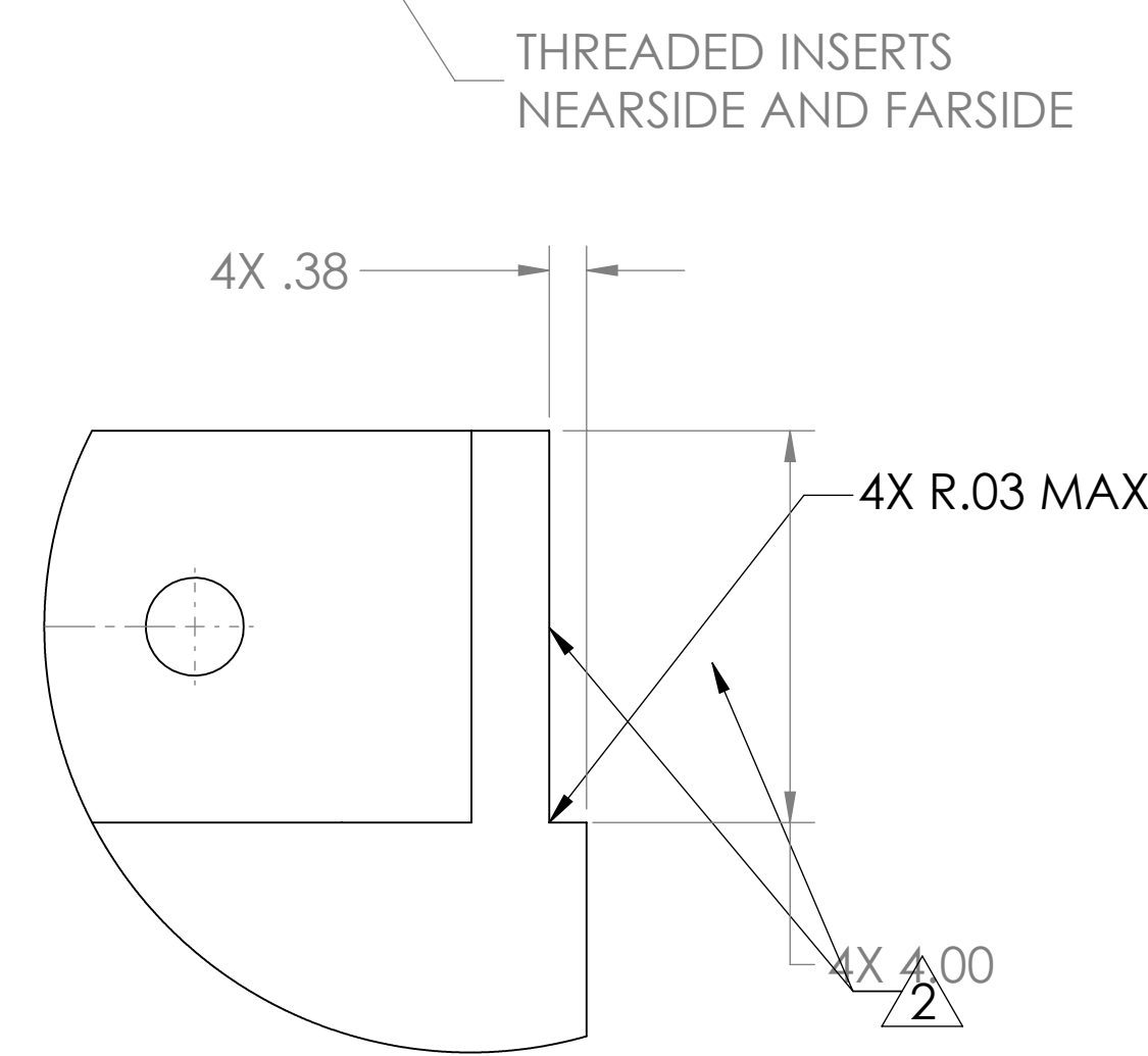
DETAIL K SCALE 1 : 2
