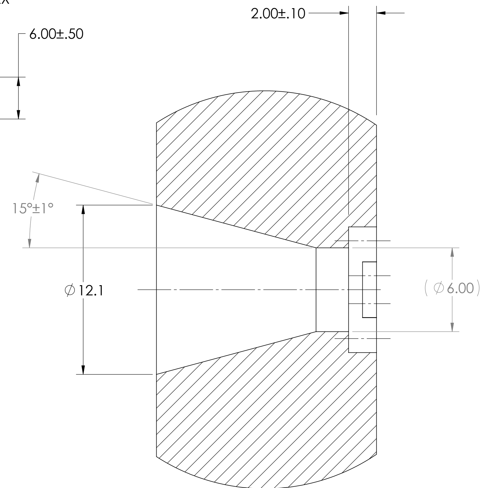
DETAIL D SCALE 1 : 4
