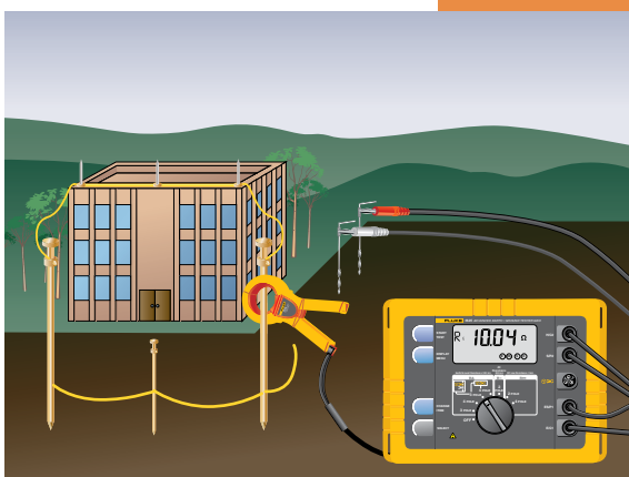
Using Selective testing on a lightning protection system.
