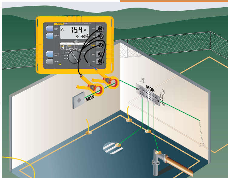
Figure 1: Stakeless testing of a central office.
