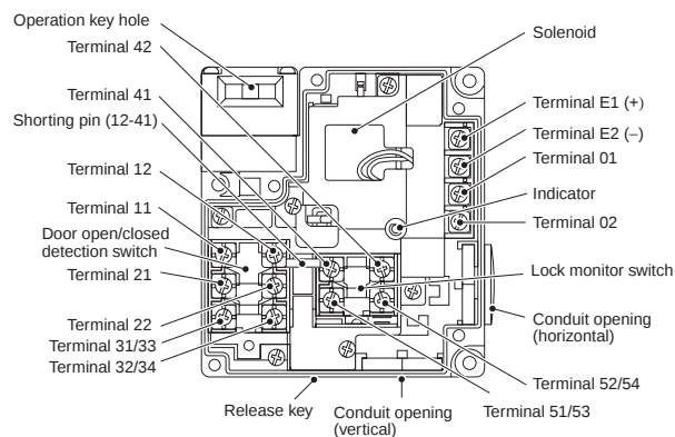
Standard Release Key (Bottom View)
