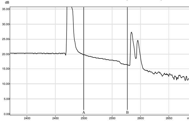
CTA-tailside-black1.trc (1310 nm)
