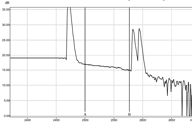
CTA-tailside-black1.trc (1550 nm)
