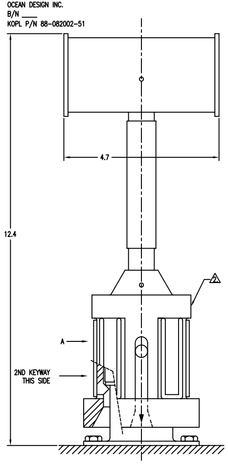
VIEW SHOWING INSTALLED CONNECTOR
