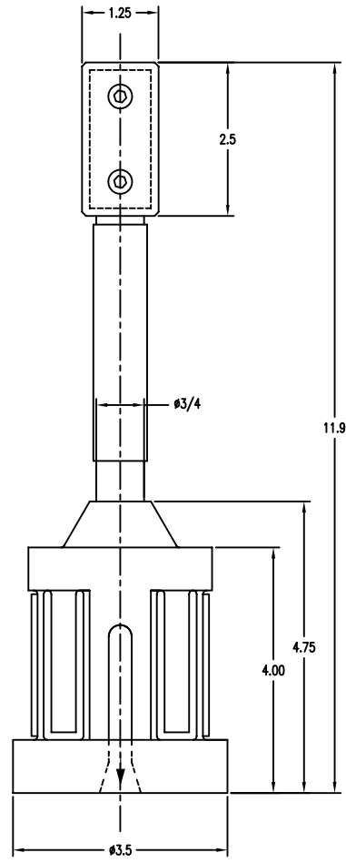
OUTLINE DIMENSIONS VIEW ON ARROW A
