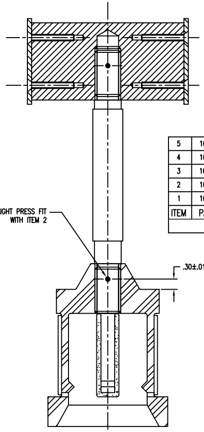
X-SECTION SHOWING ASSEMBLY INFORMATION (CAP SHELL SHOWN ROTATED 45° TO SHOW LATCHES)
