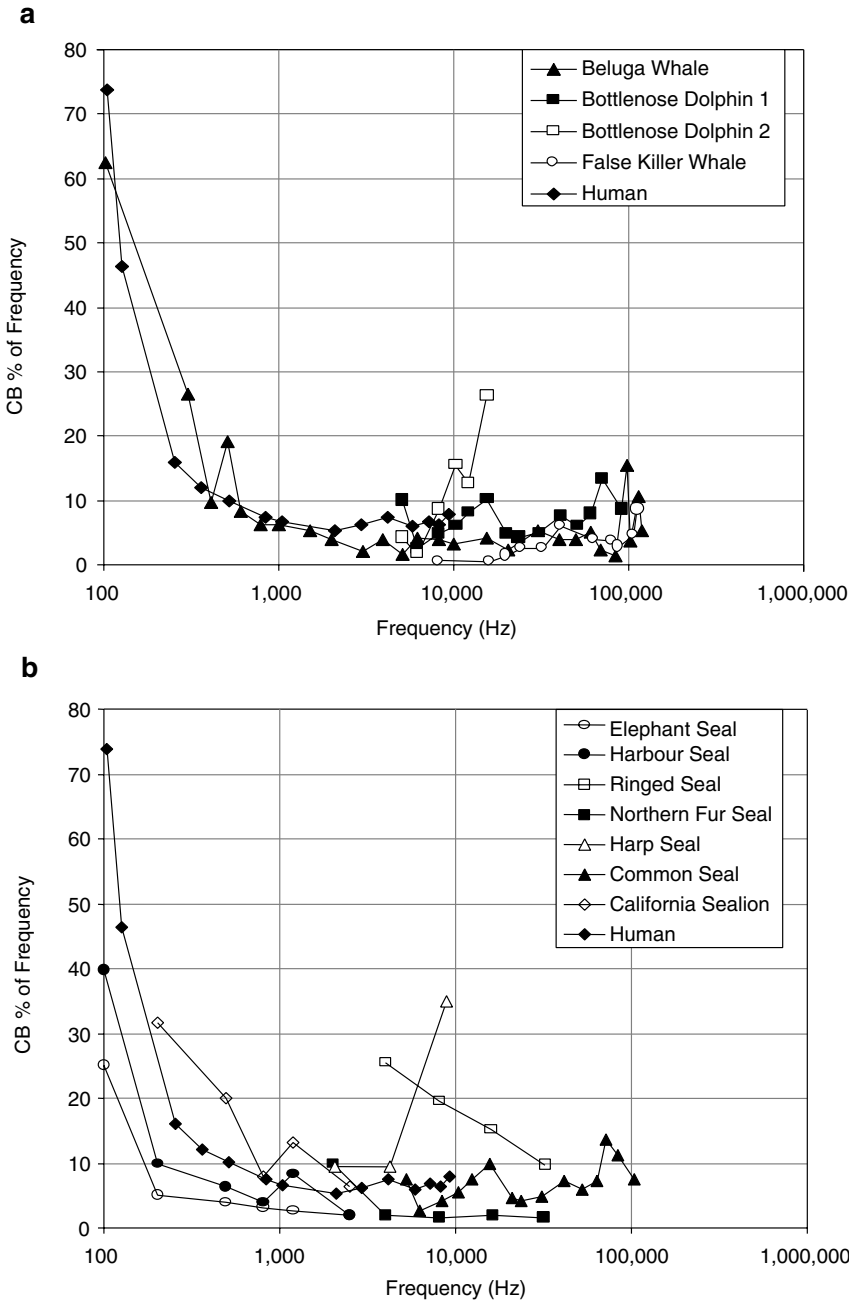
FIGURE 3-2 Critical bands of (a) odontocetes and (b) pinnipeds plotted as a proportion of frequency vs. frequency. SOURCE: Adapted from Wartzok and Ketten (1999).
