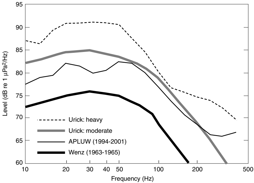
FIGURE 2-8 Point Sur autospectra compared with Wenz (1969). Point Sur data are converted to one-third octave levels and then normalized by the third-octave bandwidths for direct comparison. Shown for reference are the “heavy” and “moderate” shipping average deep-water curves presented by Urick. SOURCE: Andrew et al., 2002. Reprinted with permission of the Acoustical Society of America.
