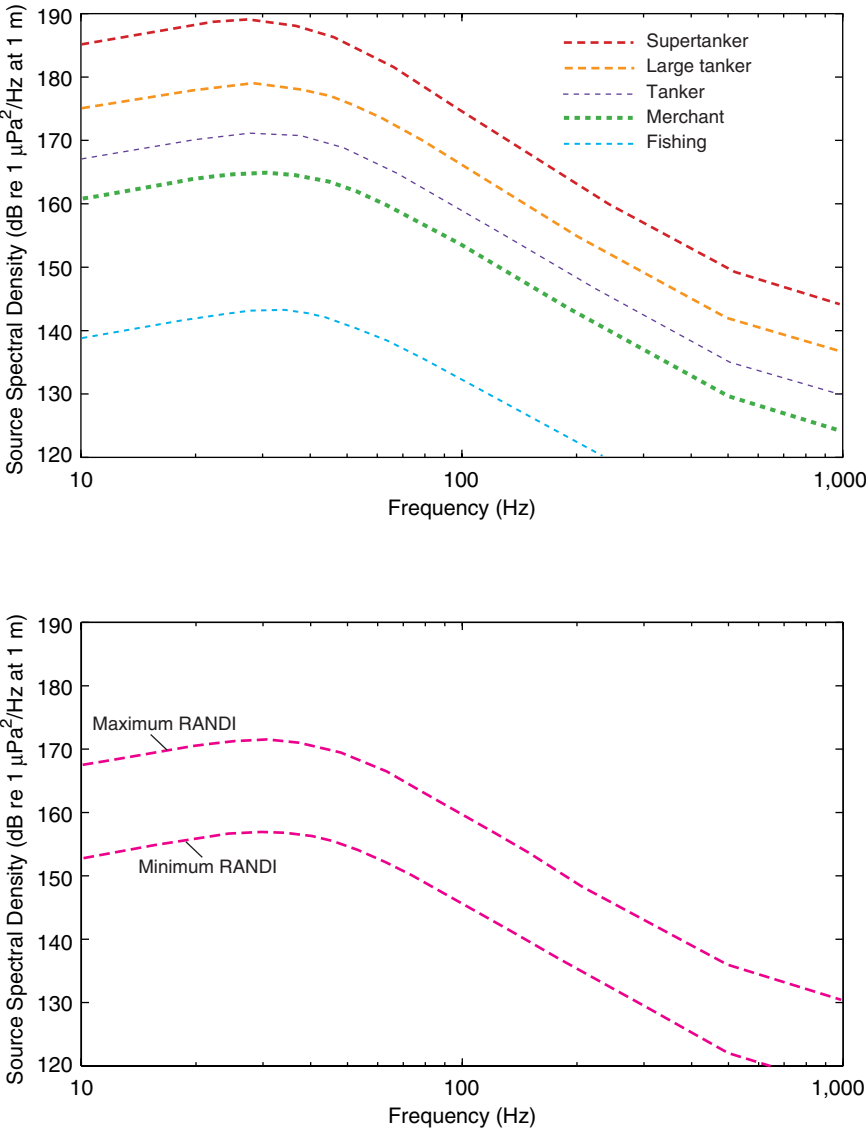
FIGURE 2-2 (a) Modeled surface ship source spectral densities for the five classes of ships used in the RANDI ambient noise model. The curves in each class also are a function of ship length and ship speed; those plotted in the figure pertain to the mean values of ship length and ship speed in each class. (b) A comparison of the maximum and minimum merchant ship source spectral densities from the RANDI model (calculated using the maximum and minimum ship lengths and ship speeds for this class; re Table 2-3). SOURCE: Wagstaff, 1973. Adapted from data from the Naval Undersea Center.
