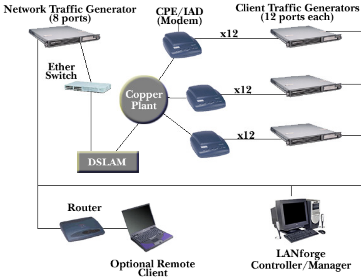
Figure 2: LANforge testing a DSL System
