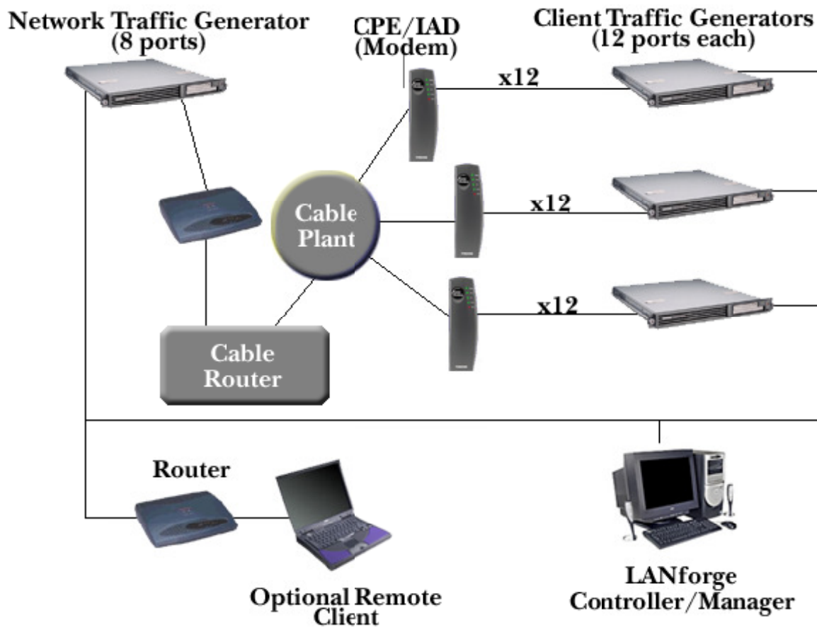
Figure 3: LANforge testing a Cable Access System
