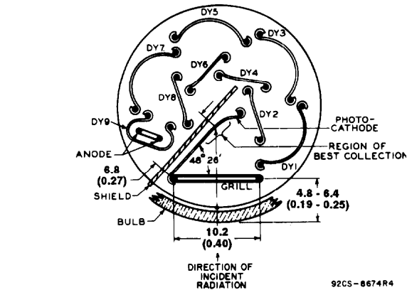
Figure 12 - Construction Detail - Top View
