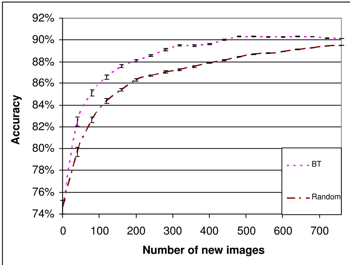
Figure 11: Unequal prior experiment. The ratio among the three classes are 1:2:4. The error bars represent the standard errors.
