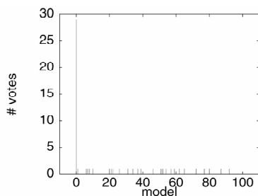
Fig. 5. Result of applying semilocal constraints: The number of votes is displayed for each model image. Semilocal constraints decrease the probability of false votes. Image 0 is recognized much more distinctively than in Fig. 3.
