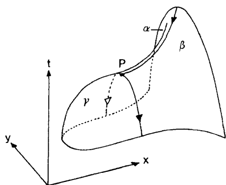
Fig. 1. The surface K = A_0 . The point P is (x_0, y_0, t_0) . In the regions alpha and beta the lines of steepest descent have the singular paths through P as asymptotes. In the region gamma these lines issue from P . Surfaces K = A_1 with A_1 > A_0 have extrema nor saddle points, whereas surfaces K = A_2 with A_2 < A_0 have one extremum and one saddle point: at point P you have a "collision" of a saddle and an extremum
