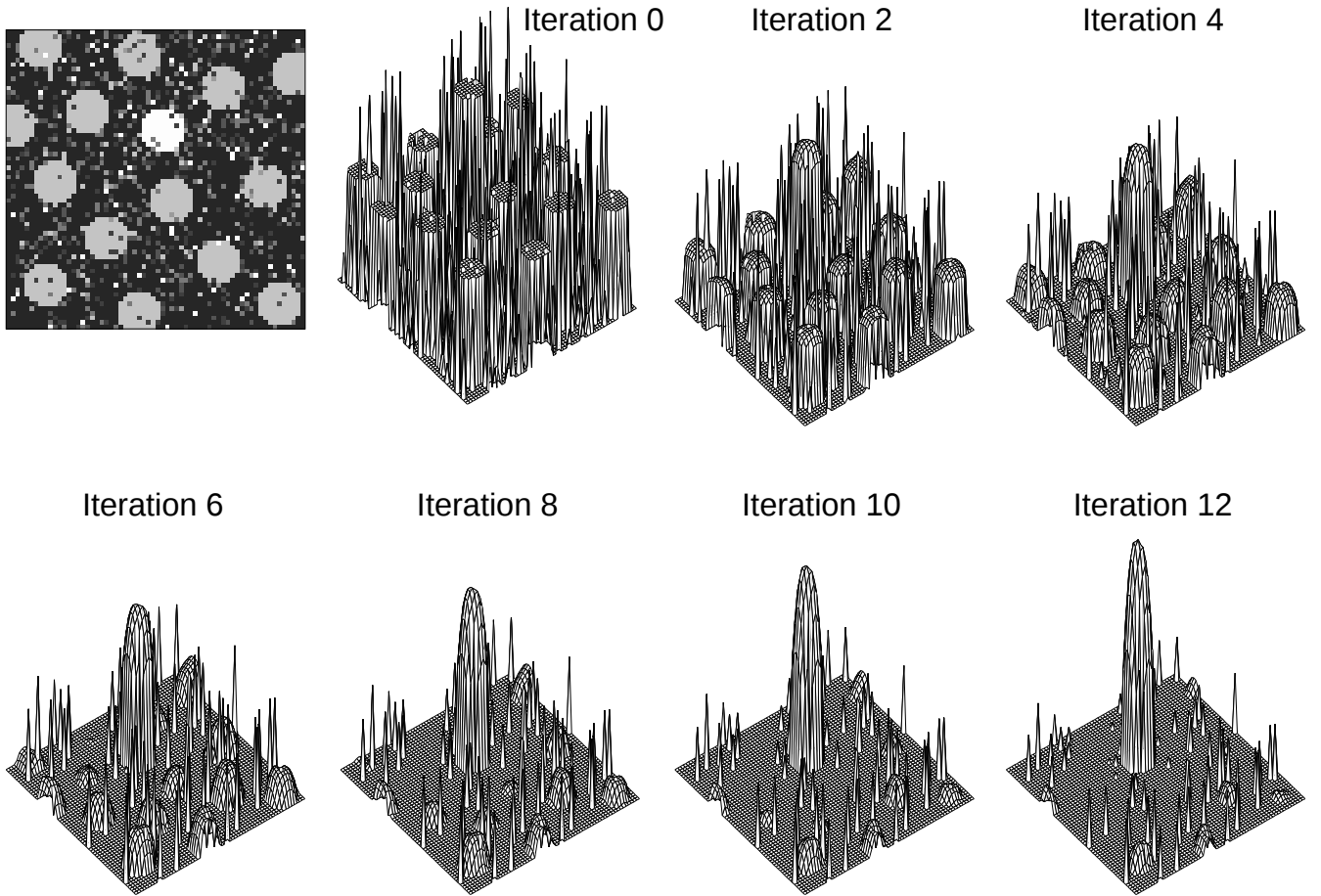
Figure 5. Iterative normalization of a feature map containing one strong activation peak surrounded by several weaker ones. After a few iterations, the initially stronger peak has gained in strength while at the same time suppressing weaker activation regions.
