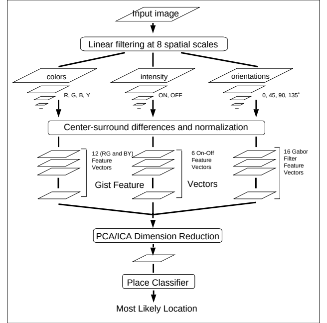
Figure 1: Visual Feature Channel Used in the Gist Model
