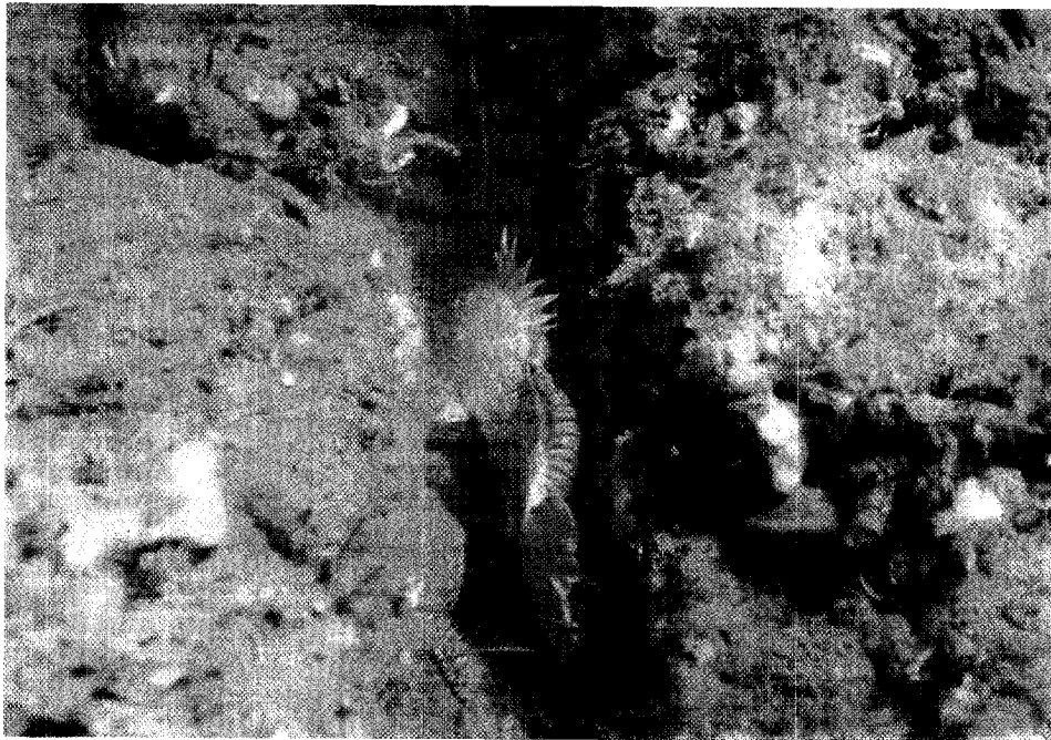
Figure 7. Crevice in the Pliocene Purisima formation that has been differentially eroded along the walls of Soquel Canyon, Monterey Bay, California. Photograph taken from the submersible Delta in 180 m water. This is typical habitat of adult greenspotted rockfishes ( Sebastes chlorostictus ).
