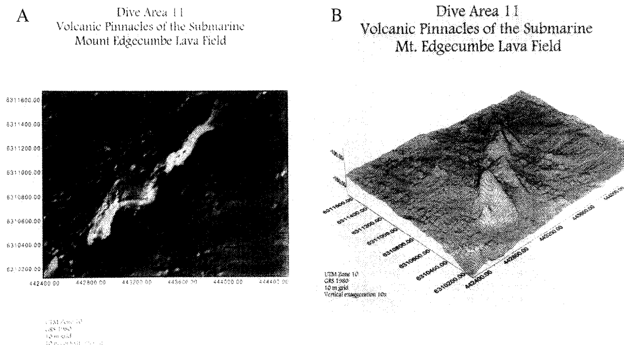
Figure 8. Bathymetric (a) shaded-relief and (b) net mesh diagrams of pinnacle (volcanic cones) mesohabitats located on the southern end of the offshore Edgecumbe lava field off Sitka, Alaska. Images produced from AMS 150 kHz side scan sonar.
