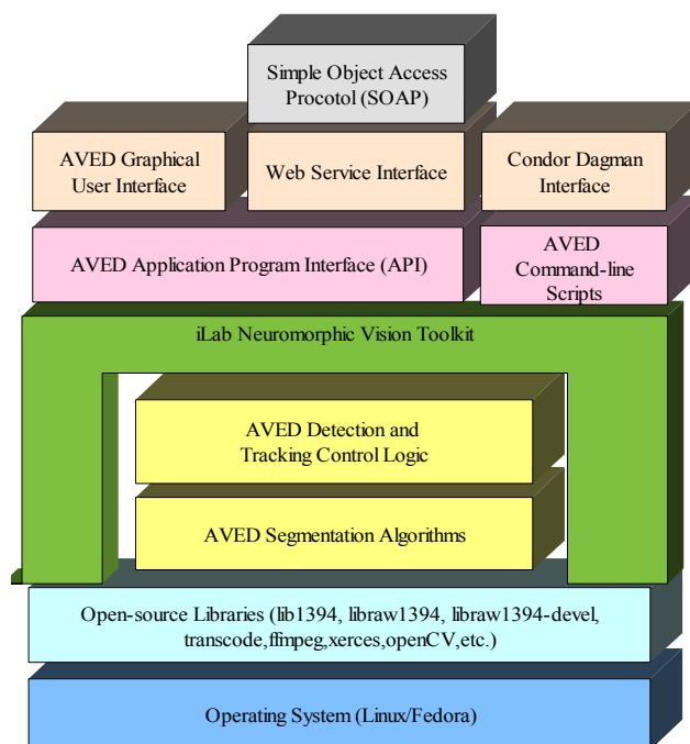
Figure 1 AVED Software Layers
