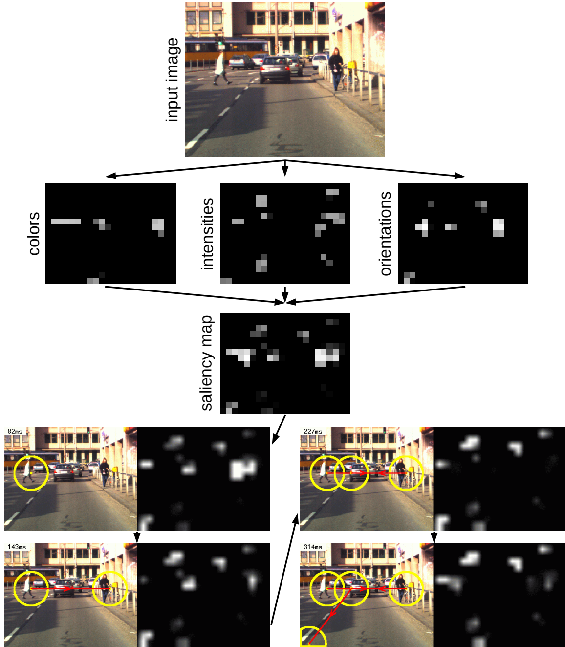
Figure 2. Example of operation of the model with a natural (color) image and the iterative feature combination strategy (see Section 2.4). The most salient location is at one pedestrian, who appears strongly in the orientation maps; it becomes the object of the first attentional shift (82 ms simulated time) and is subsequently suppressed in the saliency map by an “inhibition-of-return” mechanism. The next attended location is at another pedestrian (143 ms) which appeared strongly in the orientation and intensity maps, followed by a car (227 ms) and a street marking (314 ms). The inhibition-of-return is only transiently activated in the saliency map, such that the first attended location has regained some activity at 314 ms. More examples of model predictions on natural and synthetic images can be found at http://www.klab.caltech.edu/~itti/attention/
