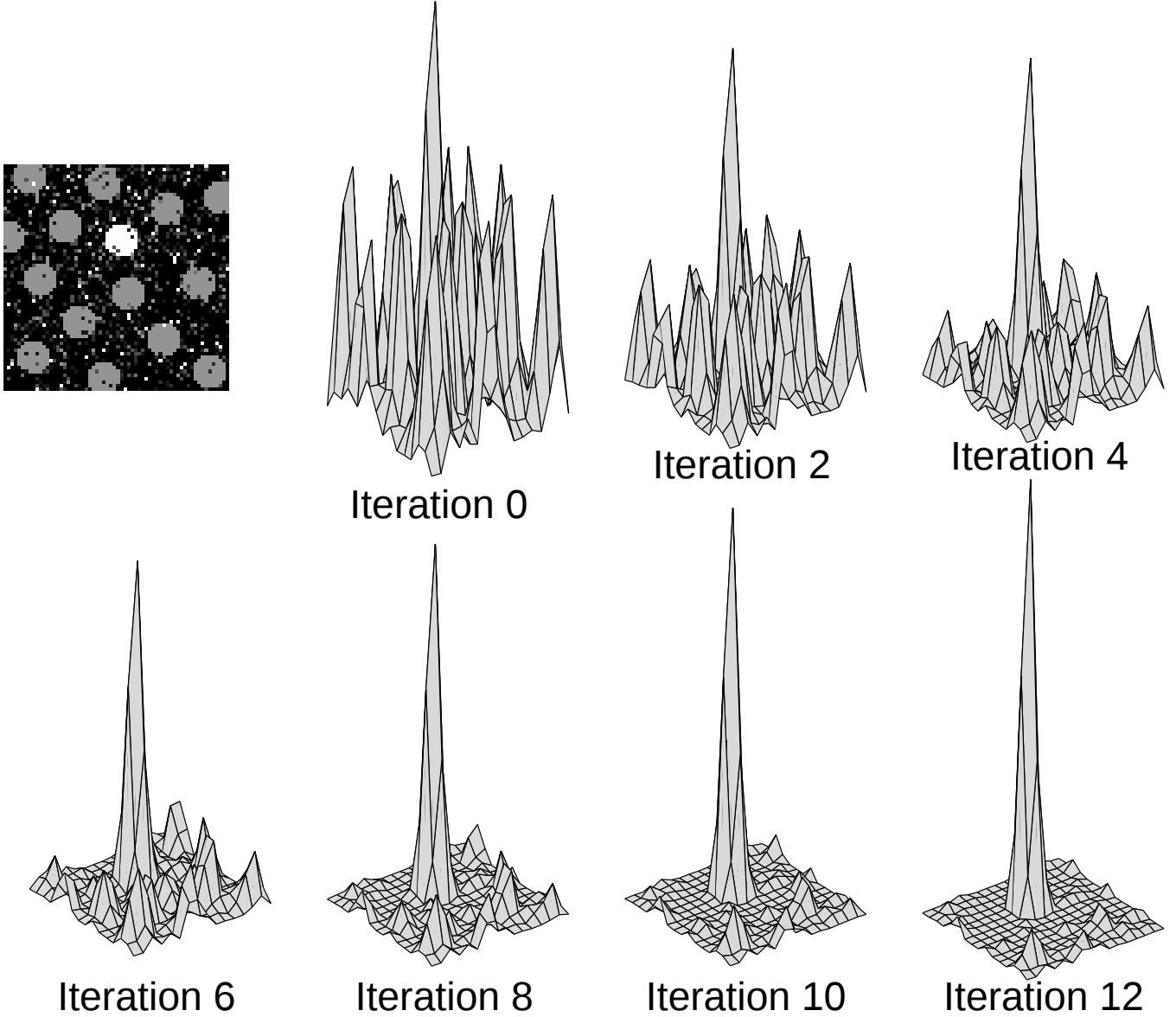
Figure 5. Iterative normalization of a feature map containing one strong activation peak surrounded by several weaker ones. After a few iterations, the initially stronger peak has gained in strength while at the same time suppressing weaker activation regions. Note how initially very strong speckle noise is effectively suppressed by the iterative rectified filtering.
