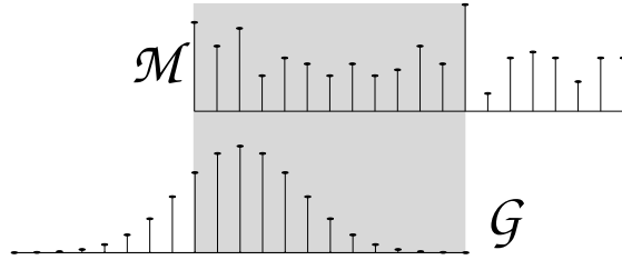
Figure 4. “Truncated filter” boundary condition consists of only computing the dot product between filter \mathcal{G} and map \mathcal{M} where they overlap (shaded area), and of normalizing the result by the total area of \mathcal{G} divided by its area in the overlap region.
