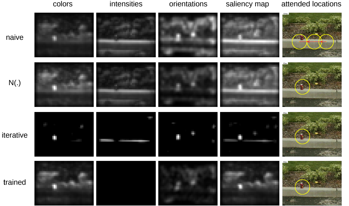
Figure 8. Comparison of the internals of the four versions of the model, for one image from the “red can” test set, in which a red aluminum can is the most salient object. The can appears with medium strength in the color maps, due to its color contrast with the background (the response is not the strongest possible because the background is not green, and only red/green and blue/yellow color contrasts are computed). The curb however appears very strongly in all intensity maps, and also less strongly in the horizontal orientation maps. In the naive version of the model, the color activity from the can is outnumbered by the activity elicited by the curb in a larger number of intensity and orientation maps. As a result, detection of the can is accidental, while the model is scanning the curb. The \mathcal{N}(\cdot) strategy yields strong suppression of the horizontal orientation, because more localized activation peaks exist in the vertical orientation, as well as some suppression of the extended curb in the intensity channel. The color channel, with its strong singularity, is however globally enhanced and yields correct detection of the can. The iterative strategy yields complete suppression of the horizontal orientation as well as overall much suppression of all regions which are not among the few strongest in each feature map. The red can clearly becomes the most salient location in the image. Finally, training using other images with similar views of this red target of vertical orientation has entirely suppressed the intensity and horizontal orientations, such that the saliency map is dominated by the color channel. The trained model hence easily finds the can as the most salient object.
