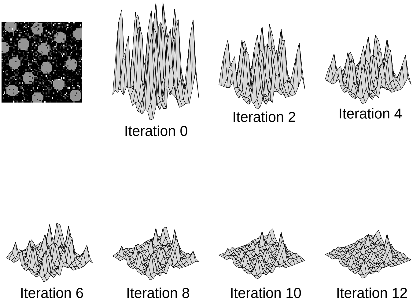
Figure 6. Iterative normalization of a feature map containing numerous strong activation peaks. This time, all peaks equally inhibit each other, resulting in the entire map being suppressed.
