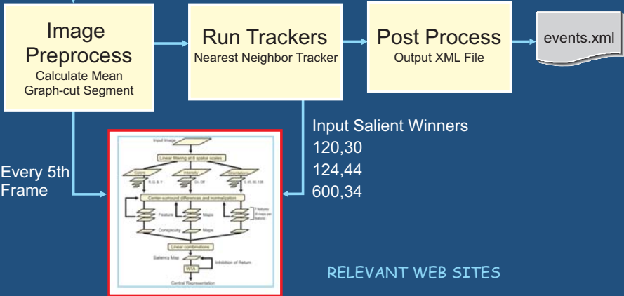
Saliency Attention Model
