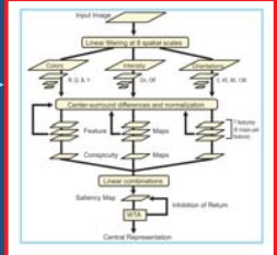
Saliency Attention Model
