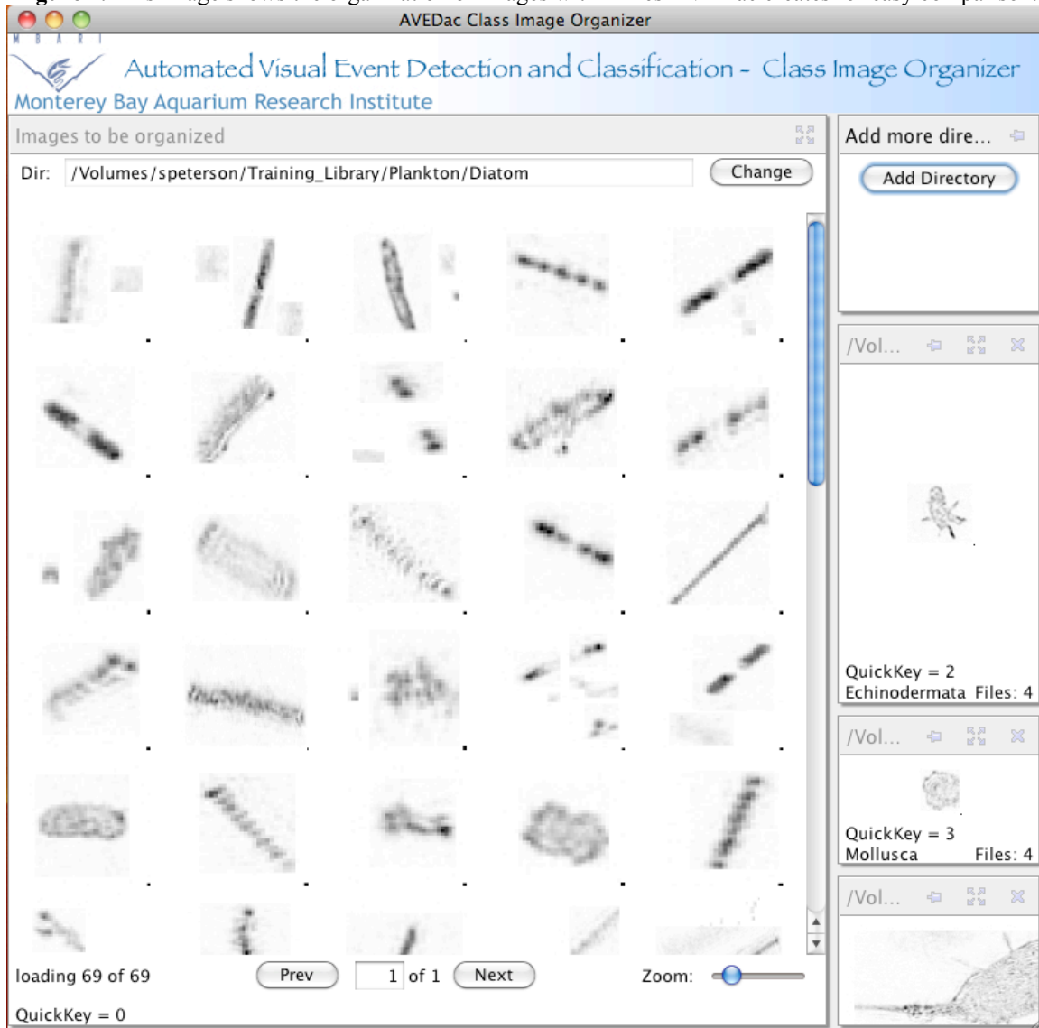
Figure 2. This image shows the organization of images within files AVEDac creates for easy comparison.
