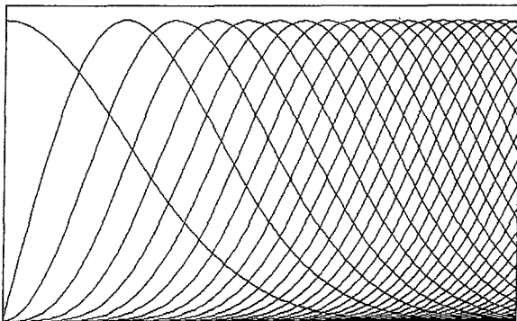
Fig. 2. Modulus of the normalized spectral transfer functions of the RF's plotted on linear scales
