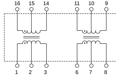
Schematic A
