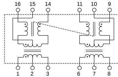
Schematic B
