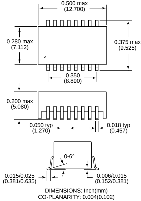
SMD Package
