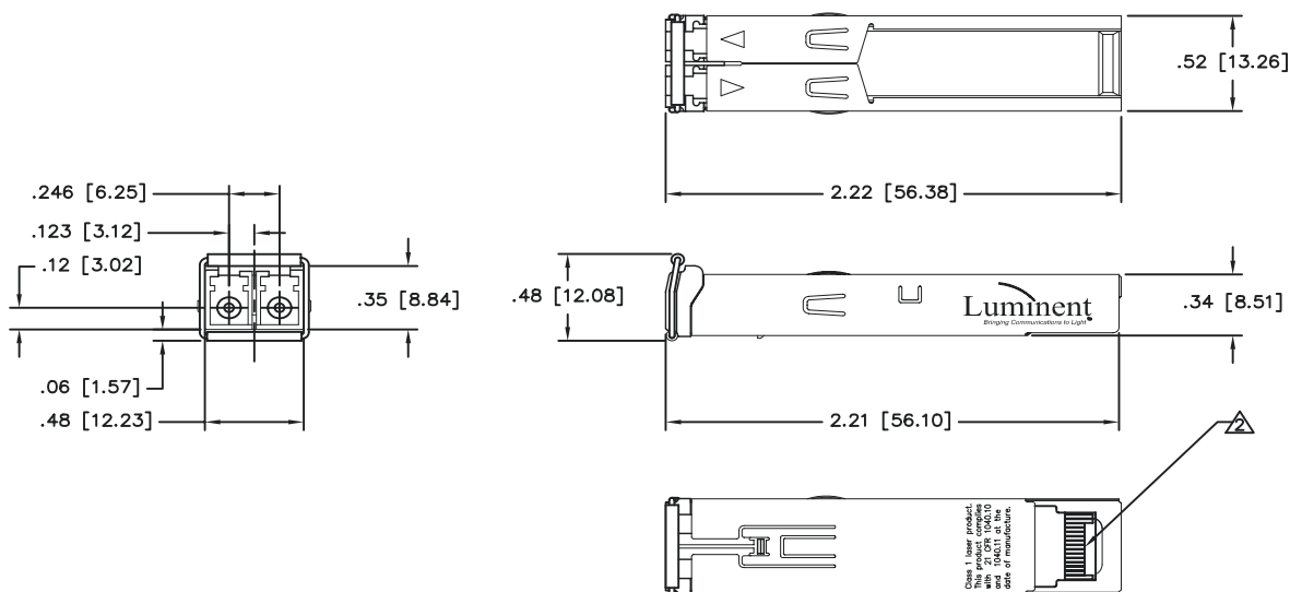
Outline Drawing (Bail Latch)
