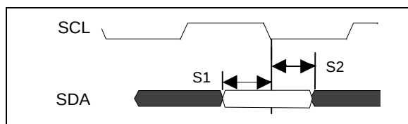
Figure 23 - I 2 C Input Setup Timing
