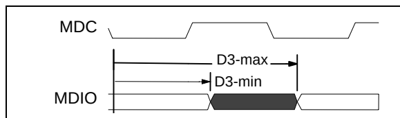
Figure 22 - MDIO Output Delay Timing
