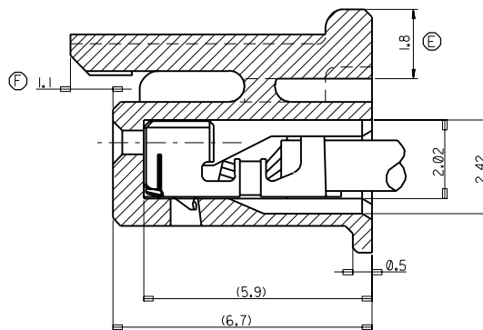
TERMINAL INSERTED DRAWING SCALE 2:1
