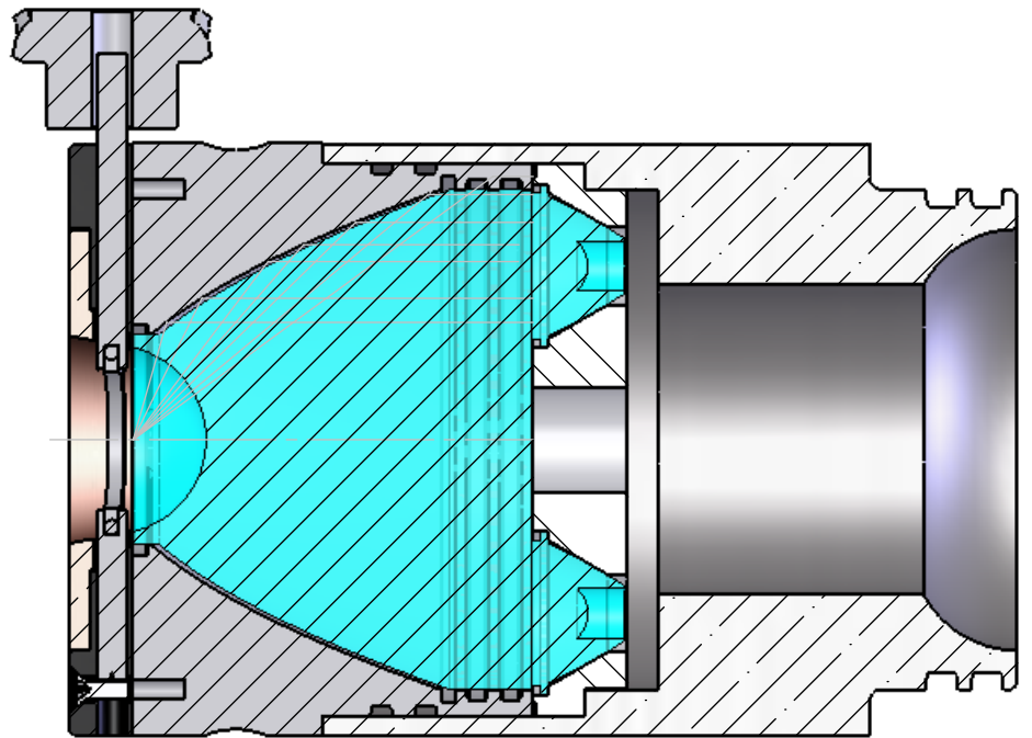
SECTION H-H
