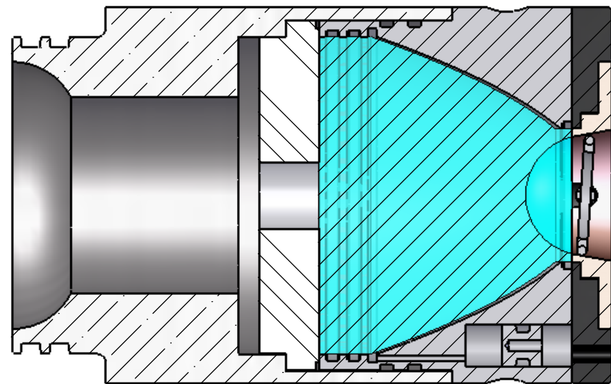
SECTION F-F
