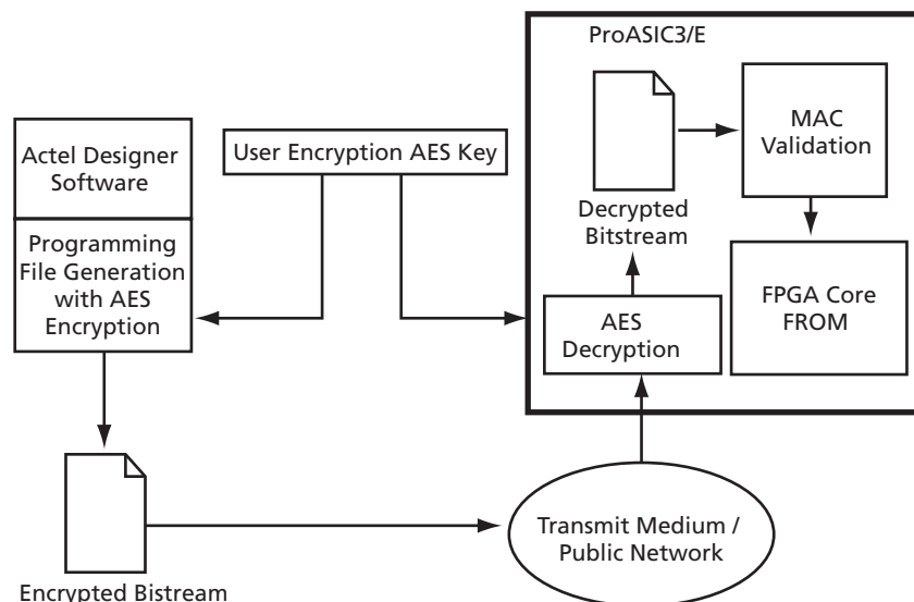
Figure 1 • AES-128 Security Features in ProASIC3/E Devices
