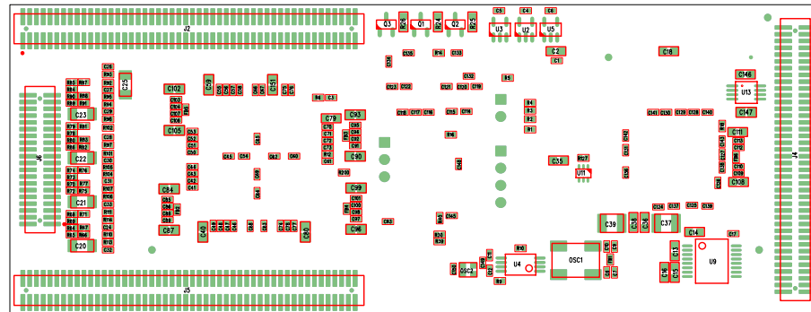
MBARI BIOSA CPU - 1002605_0 TOP ASSEMBLY
