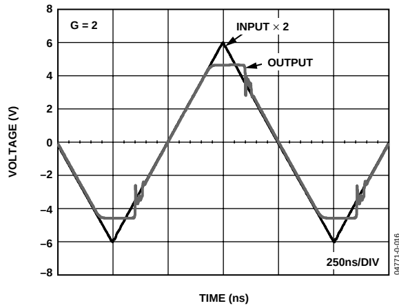
Figure 37. Overdrive Recovery
