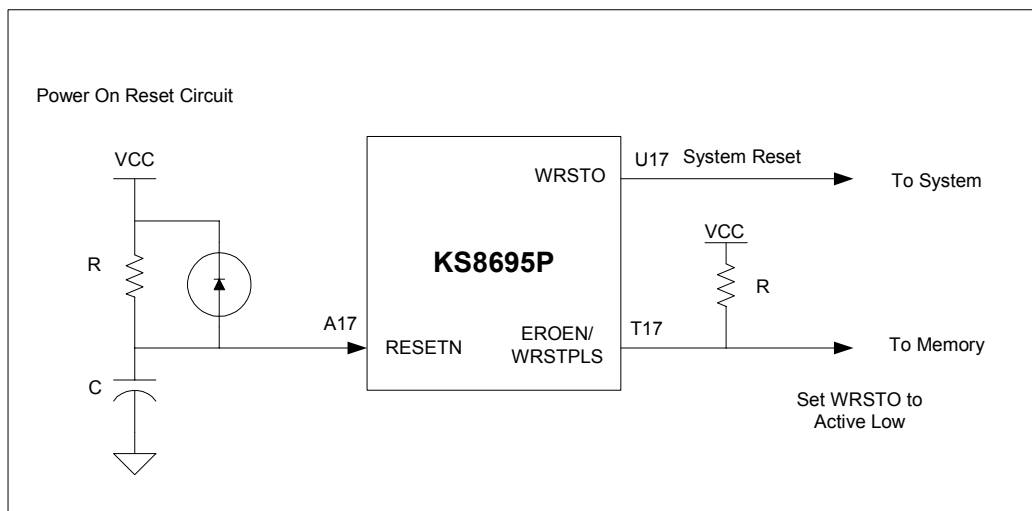
Figure 5 Example Reset Circuit
