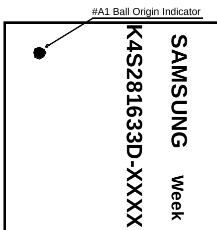
< Top View *2 >
