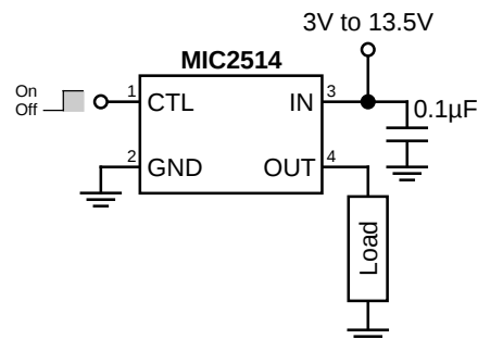
High-Side Power Switch
