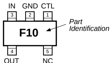
5-Lead SOT-23-5 (M5)
