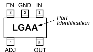
MIC5219BM5 SOT-23-5 Adjustable Voltage (Top View)
