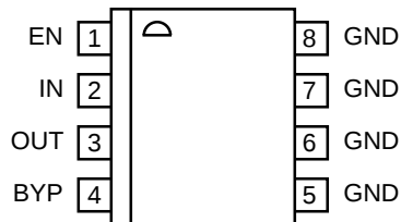
MIC5219-x.xBMM MM8™ MSOP-8 Fixed Voltages (Top View)
