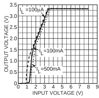
Dropout Characteristics
