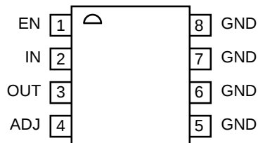
MIC5219YMM MIC5219BMM MM8™ MSOP-8 Adjustable Voltage (Top View)
