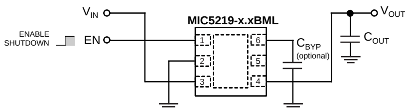
Ultra-Low-Noise Regulator
