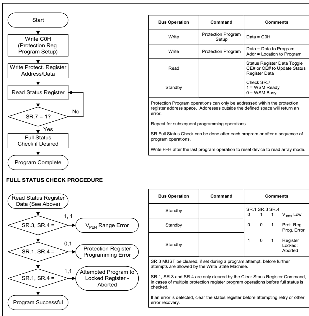
Figure 26. Protection Register Programming Flowchart
