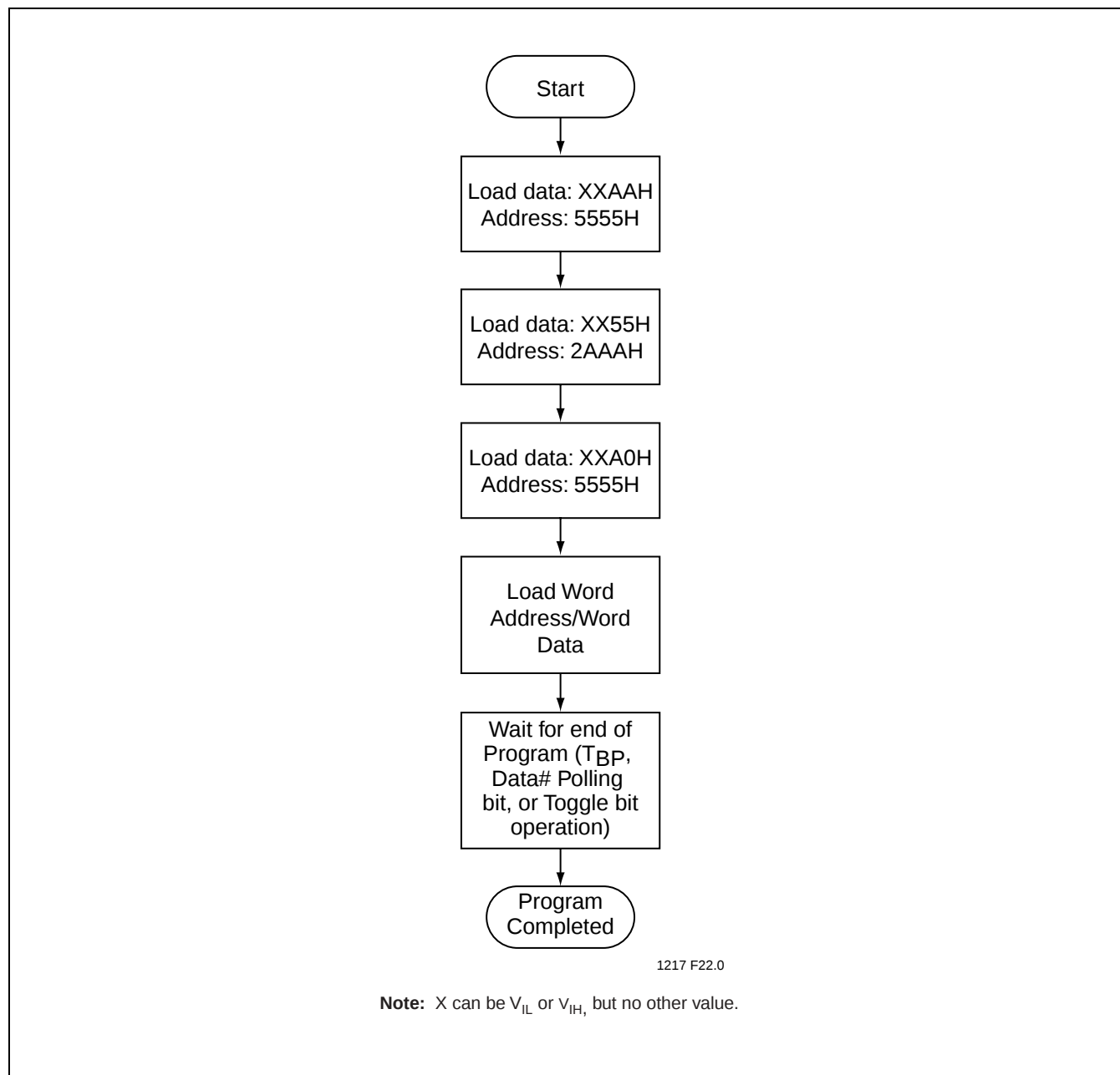
FIGURE 22: WORD-PROGRAM ALGORITHM
