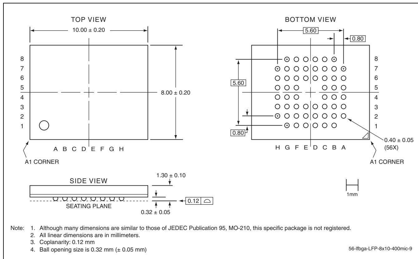
56-BALL LOW-PROFILE, FINE-PITCH BALL GRID ARRAY (LFBGA) 8MM X 10MM SST PACKAGE CODE: LFP
