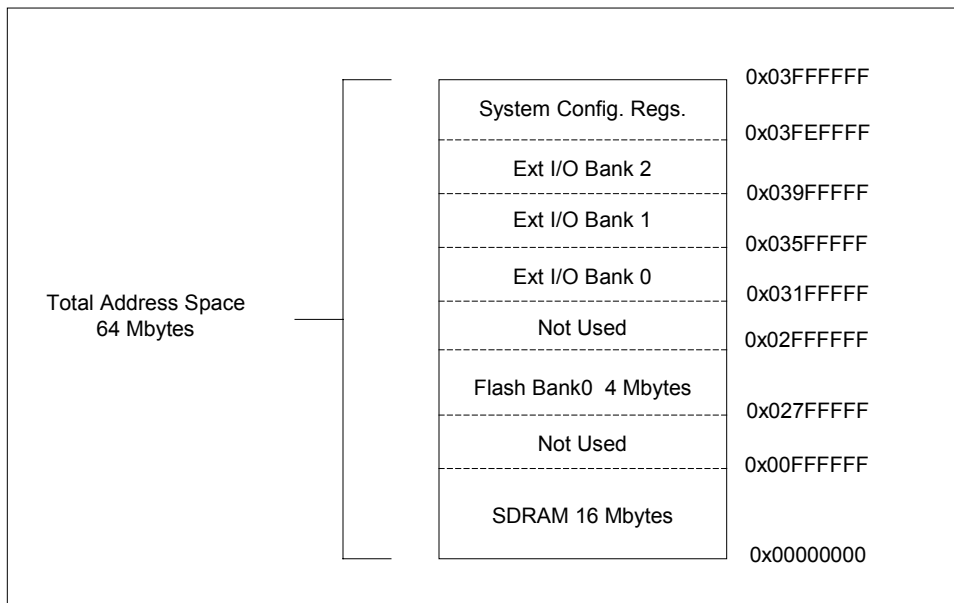
Figure 3 Memory Space Remap Example
