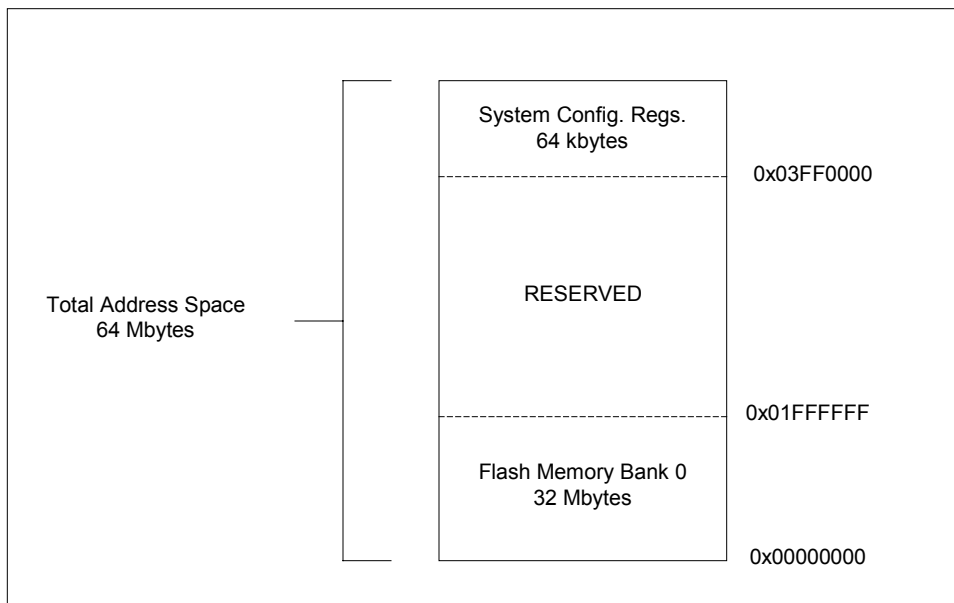
Figure 2 KS8695P Default Memory Map
