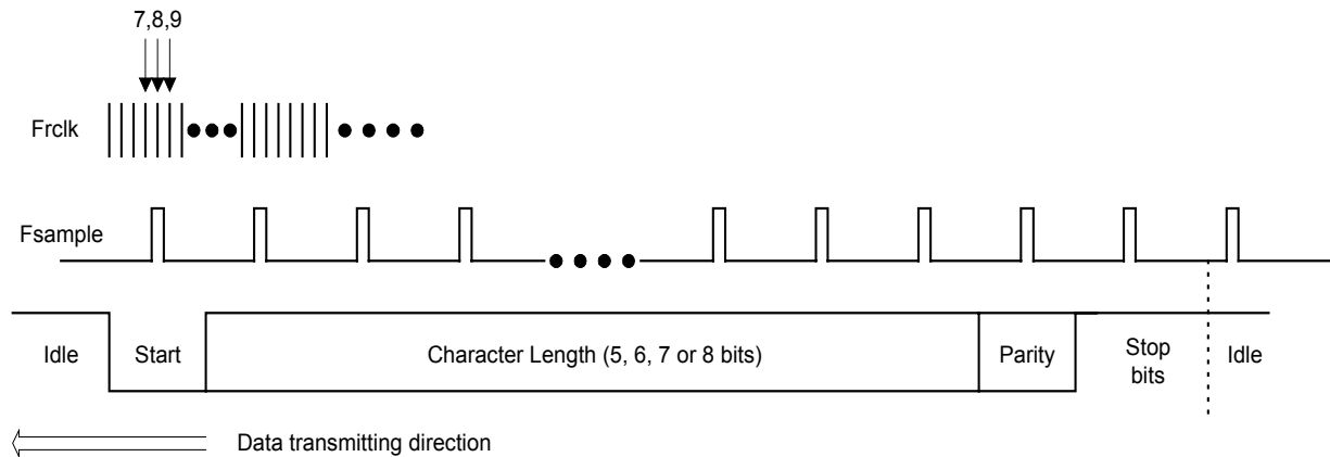
Figure 8 UART Line Control
