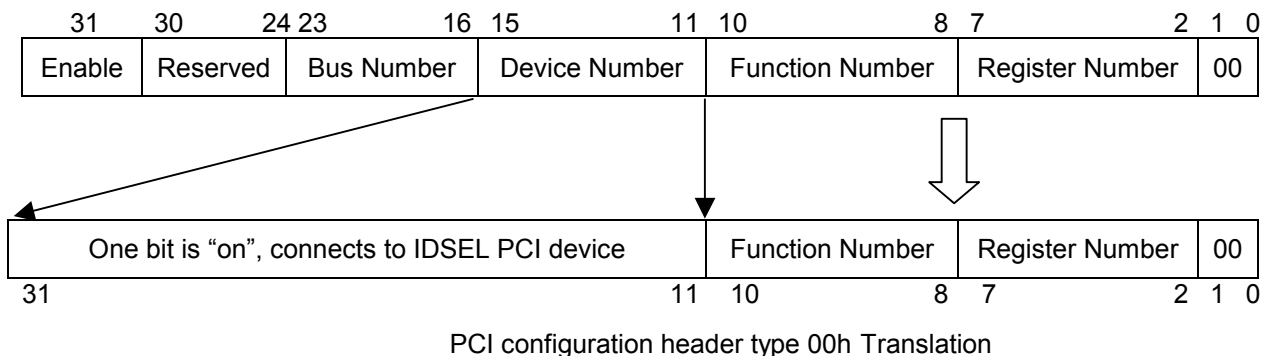
Figure 6 PCI Type 00 Configuration
