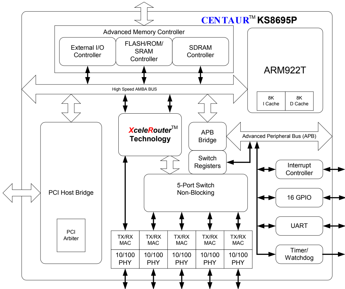
Figure 1 KS8695P Functional Block Diagram
