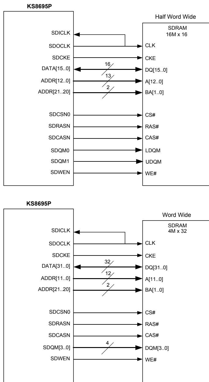
Figure 8. SDRAM Interface Examples
