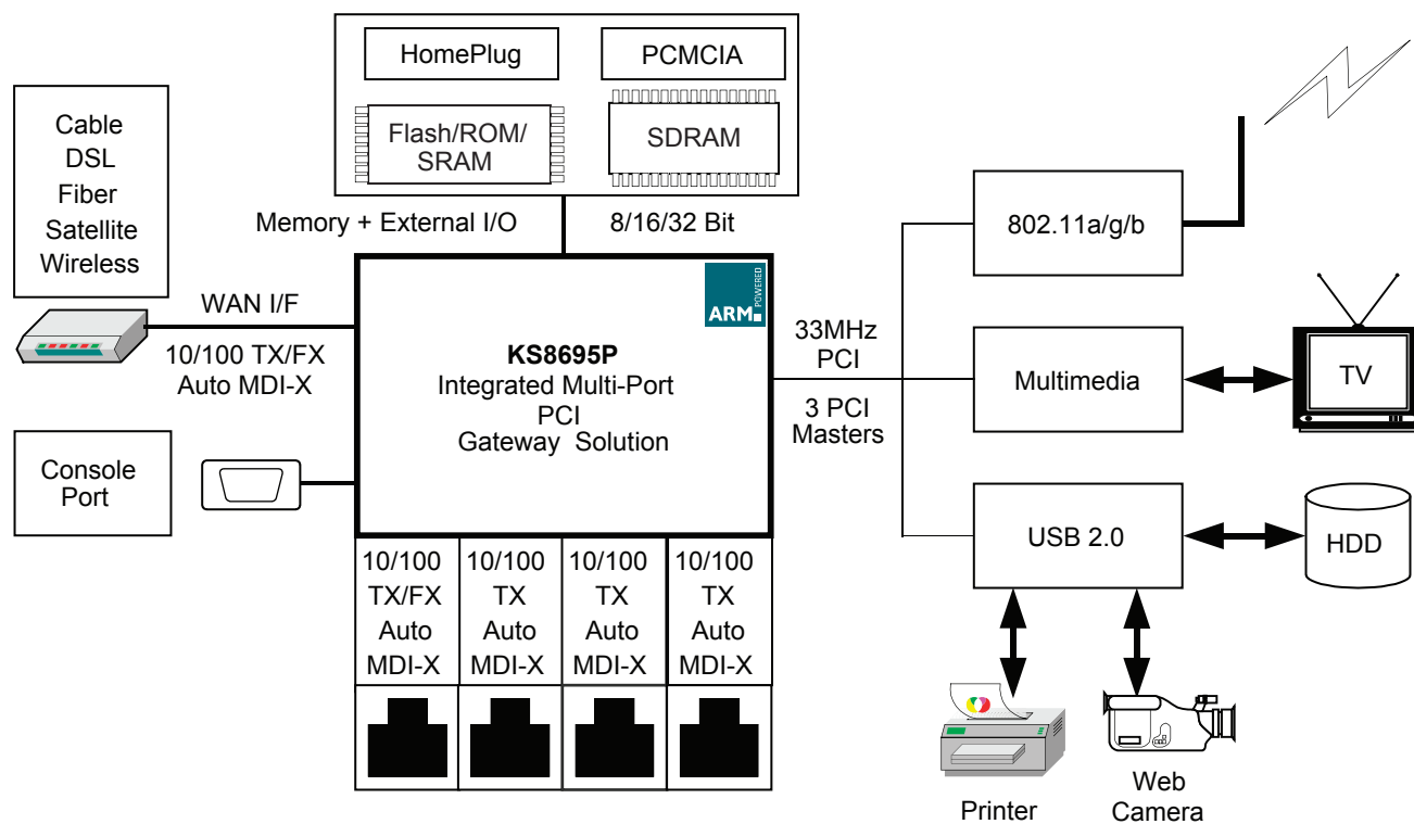
Figure 1. KS8695P PCI Gateway System Options
