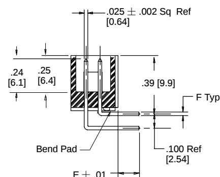
Section J-J
