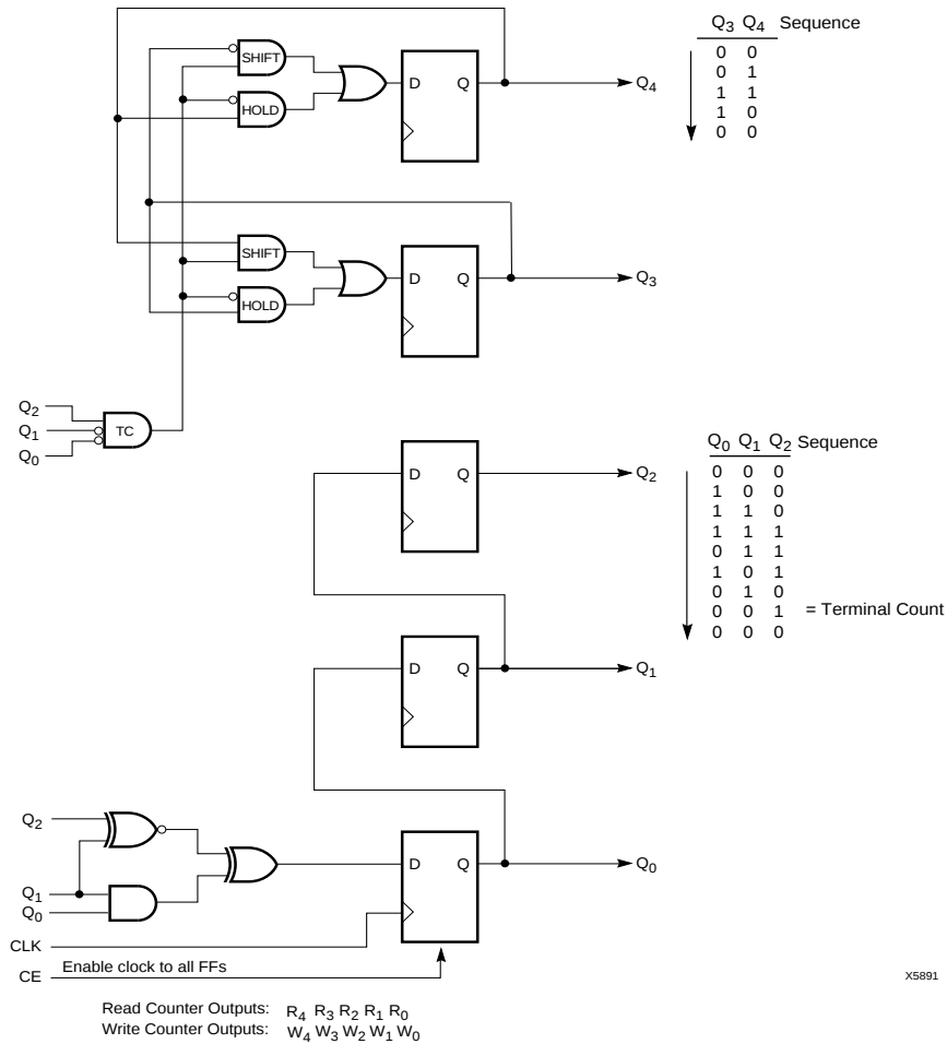
Figure 7: 32-Deep FIFO, Read Counter or Write Counter
