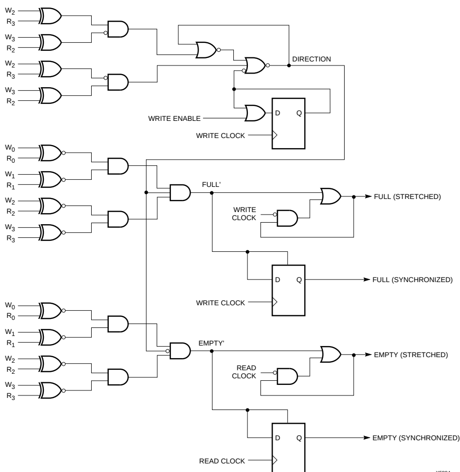
Figure 5: 16-Deep FIFO, Asynchronous Control
