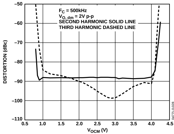
Figure 31. Harmonic Distortion vs. V_{OCM} , V_S = +5 V
