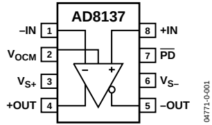
Figure 4. Pin Configuration
