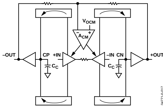
Figure 61. Block Diagram
