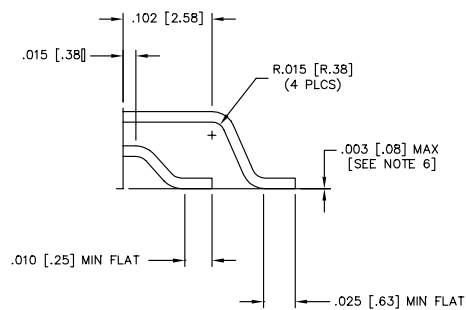
DETAIL 'A' SCALE: 2x
