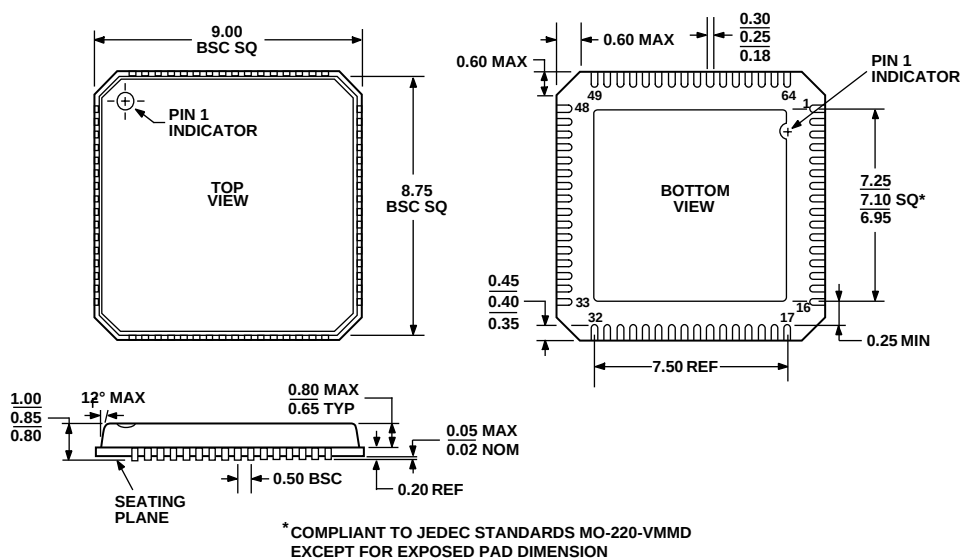
Figure 61. 64-Lead Lead Frame Chip Scale Package (LFCSP) [CP-64] Dimensions shown in millimeters
