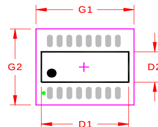
SILKSCREEN & COURTYARD
