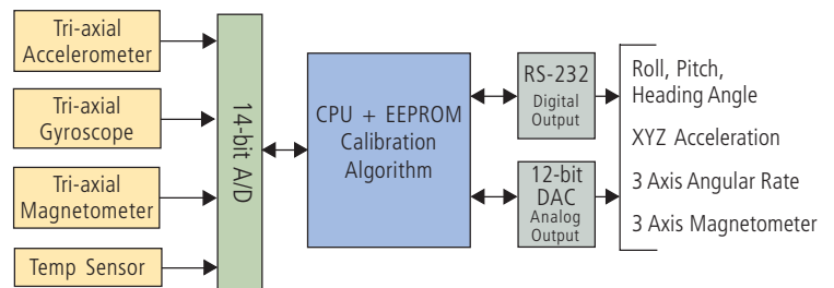
AHRS Block Diagram
