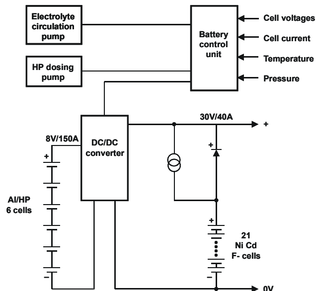
Fig. 2. The HUGIN 3000 power source.
