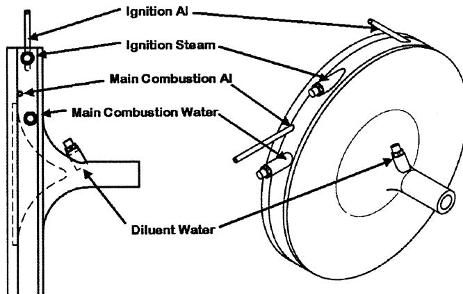
Fig. 7. Concept sketch for a low-rate/long-endurance combustor
