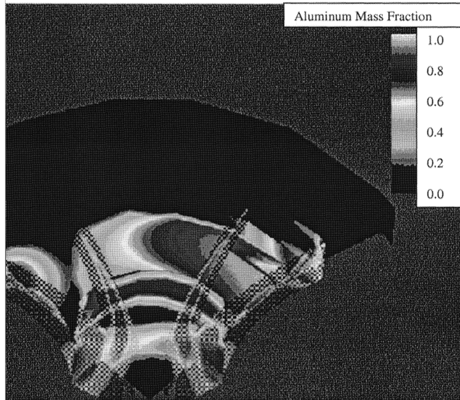
CFD calculation showing mass fraction of aluminum within a model vortex combustor chamber.
