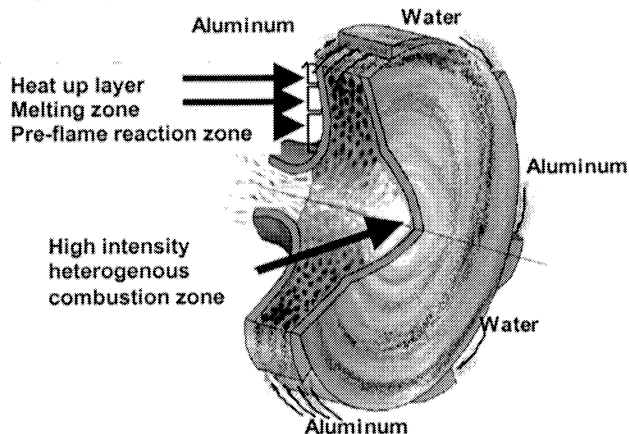
Fig. 5. Conceptual sketch of the vortex combustor flowfield.
