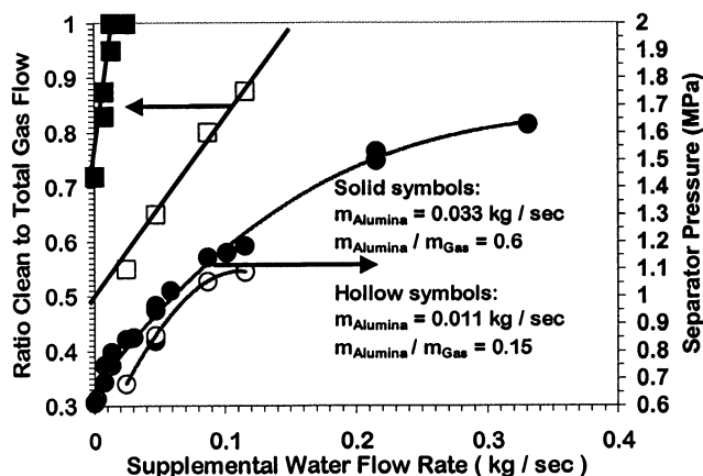
Fig. 11. Separator efficiency and pressure-drop of the particle separator as a function of supplemental water flow rate.
