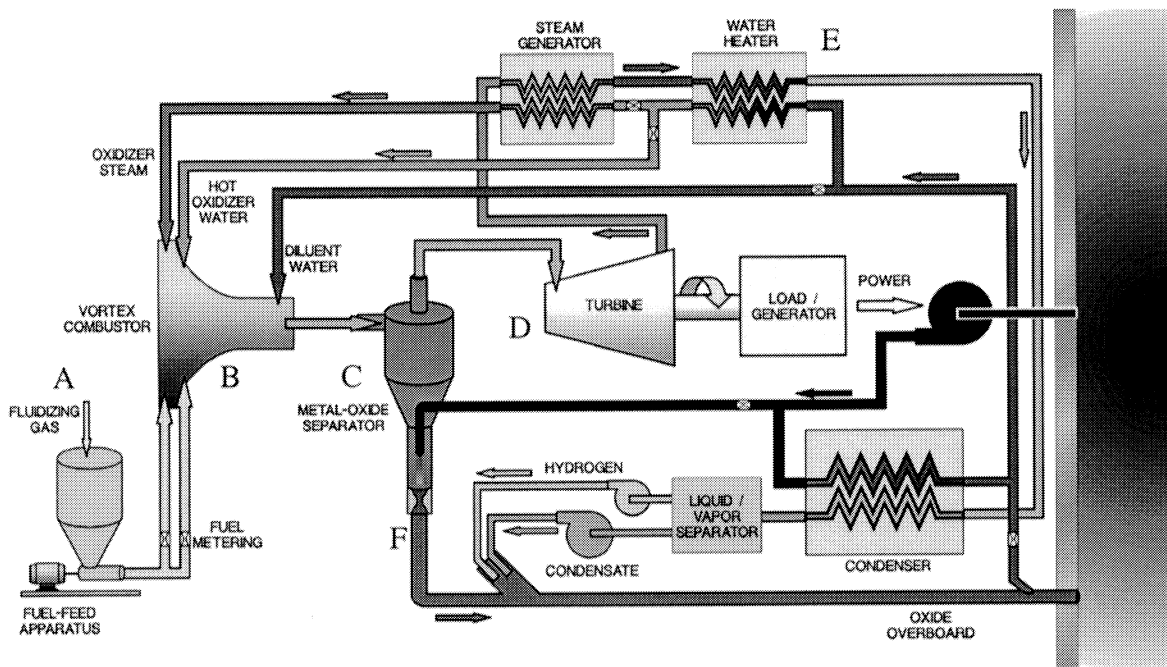
Fig.1. Sketch of Proposed Al-Seawater AUV Energy System.
