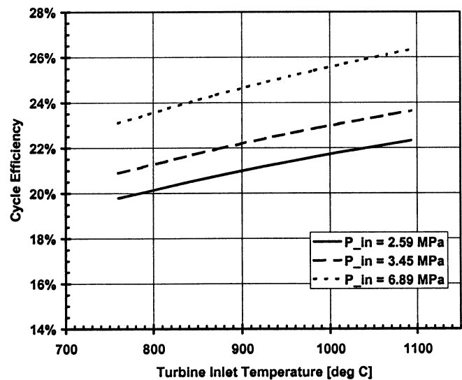
Fig. 2. Predicted cycle efficiencies for the proposed Al-seawater AUV energy system at different turbine inlet temperatures and pressures.
