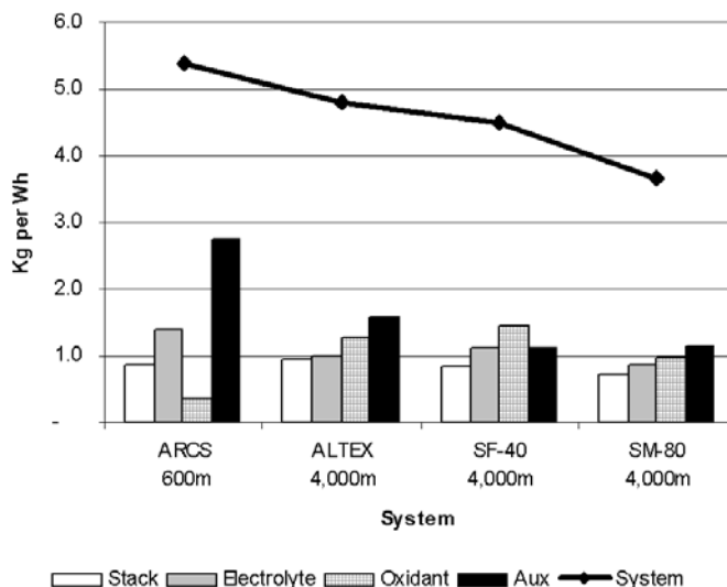
Fig. 1. Gravimetric Effectiveness Progression
