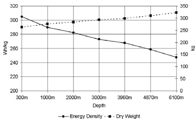
Fig. 2. Neutrally Buoyant Energy Density
