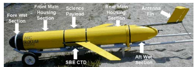
Fig. 2. Slocum Battery Glider.
