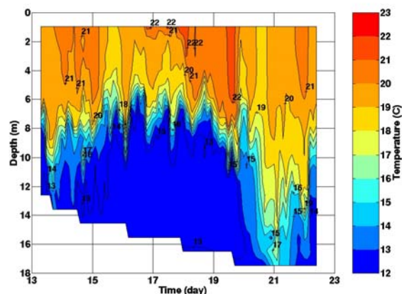
Fig. 6. Temperature data collected during the July 13-22, 2000 Glider deployment.
