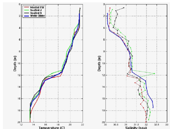
Fig. 7. Comparison of conductivity and temperature data from the Glider and shipboard CTDs.
