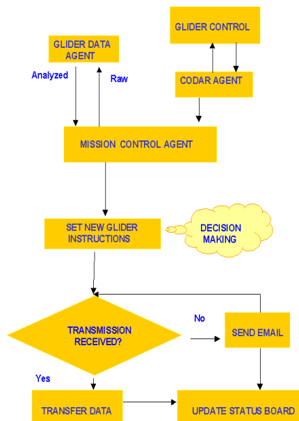
Fig. 4. Agent Flow-Chart.
