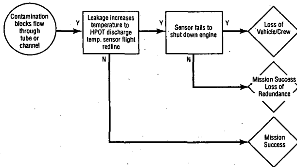
Figure 3. Example ESD
