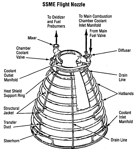
Figure 2. SSME Tube Nozzle
