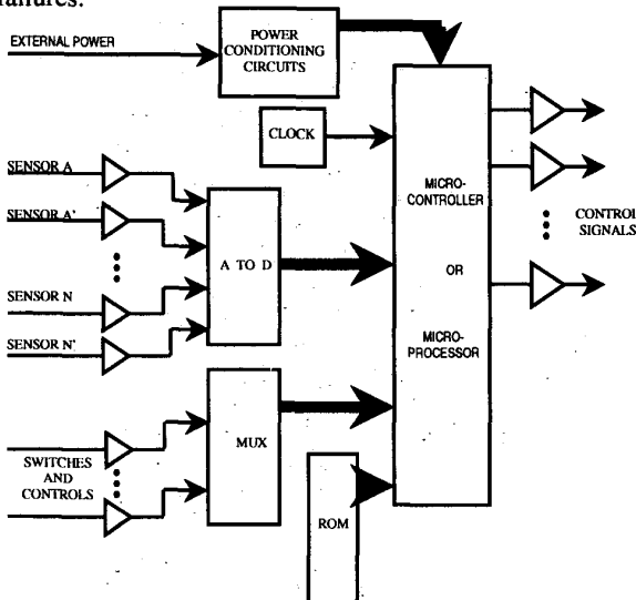
Figure 1. Hardware Architecture.
