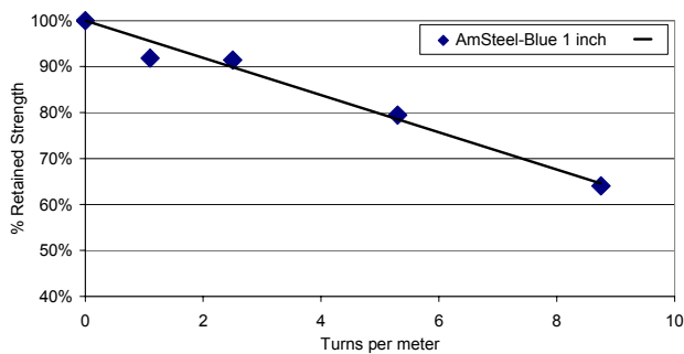
Fig. 11. Effect of twist on breaking strength
