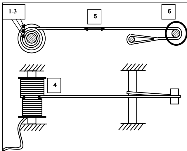
Fig. 1. Schematic of winch drum compression test.
